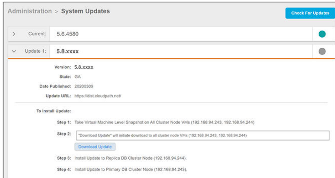
FIGURE 1 System Updates Screen for Upgrading a Cluster From 5.6.4580 to 5.8.5012
